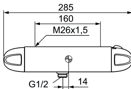
9210 Pressure Balanced Thermostatic Shower Mixer
