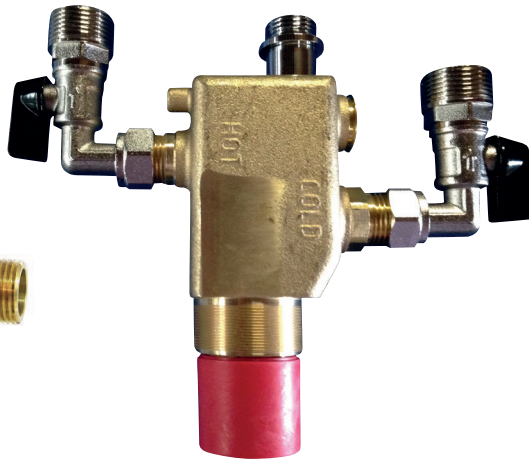
Product 9230-8071 PBTMV complete with isolating valves
