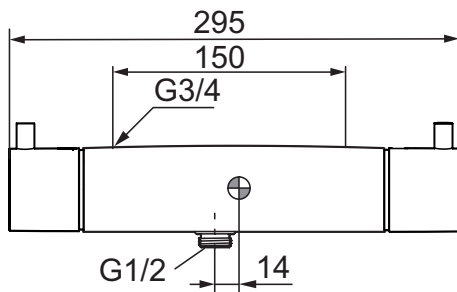
9680 Pressure Balanced Thermostatic Shower Mixer - Garda Range
